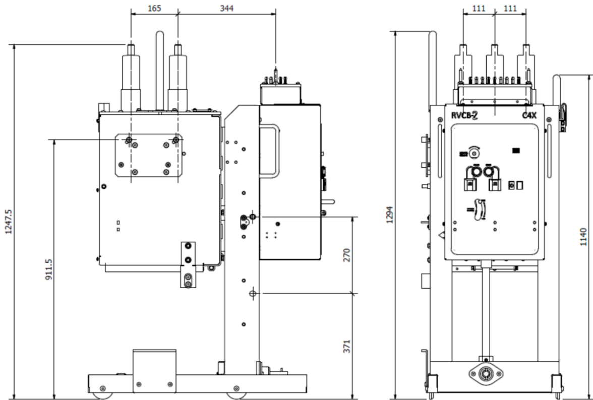
Figure 1. SWS-Lo RVCB Dimensions
